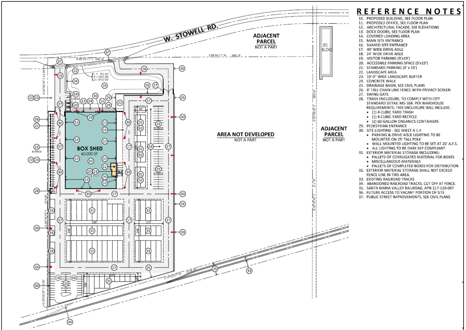
Figure 3 – Site Plan
