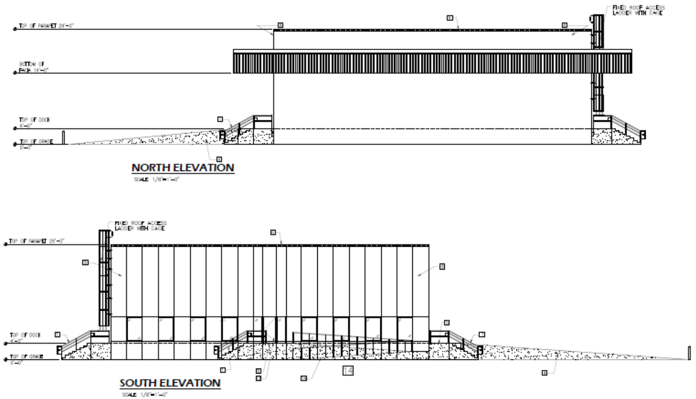
Figure 4: North and South Architectural Elevations
