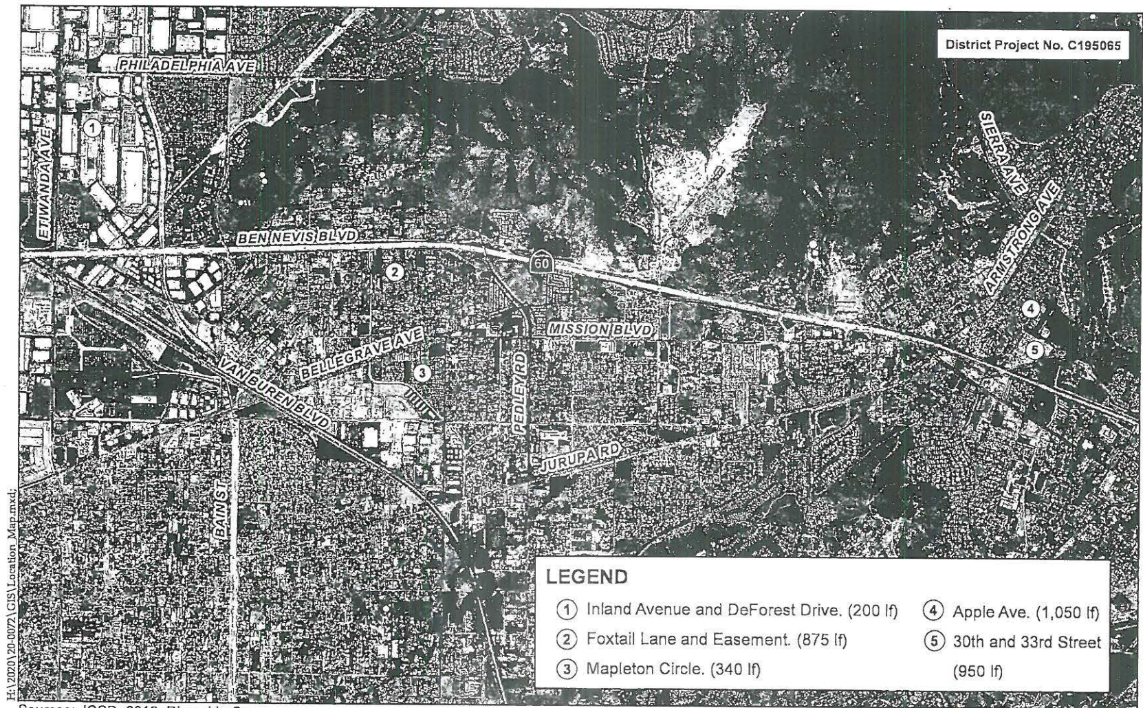
Figure 1 - Location Map JCSD FY 20-21 Sewer Replacement Project
