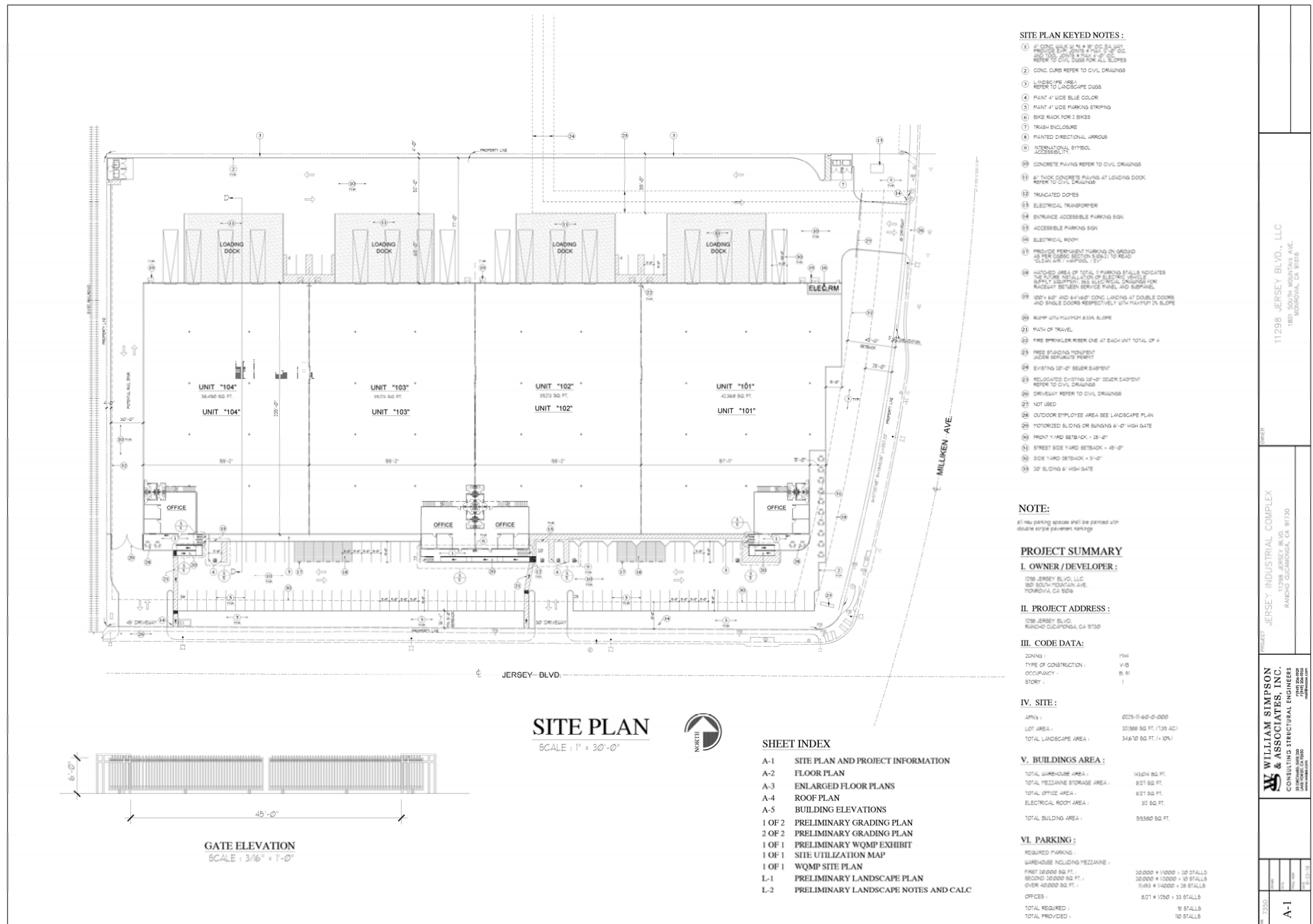
Figure 2— Site Plan
