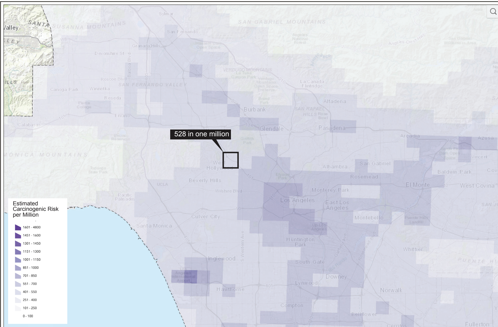
Figure IV.A-3 MATES V Total Cancer Risk for the Project Area
