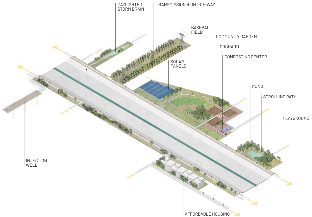
KOP 6 Off-Channel Land Assets (Trapezoidal Channel)
