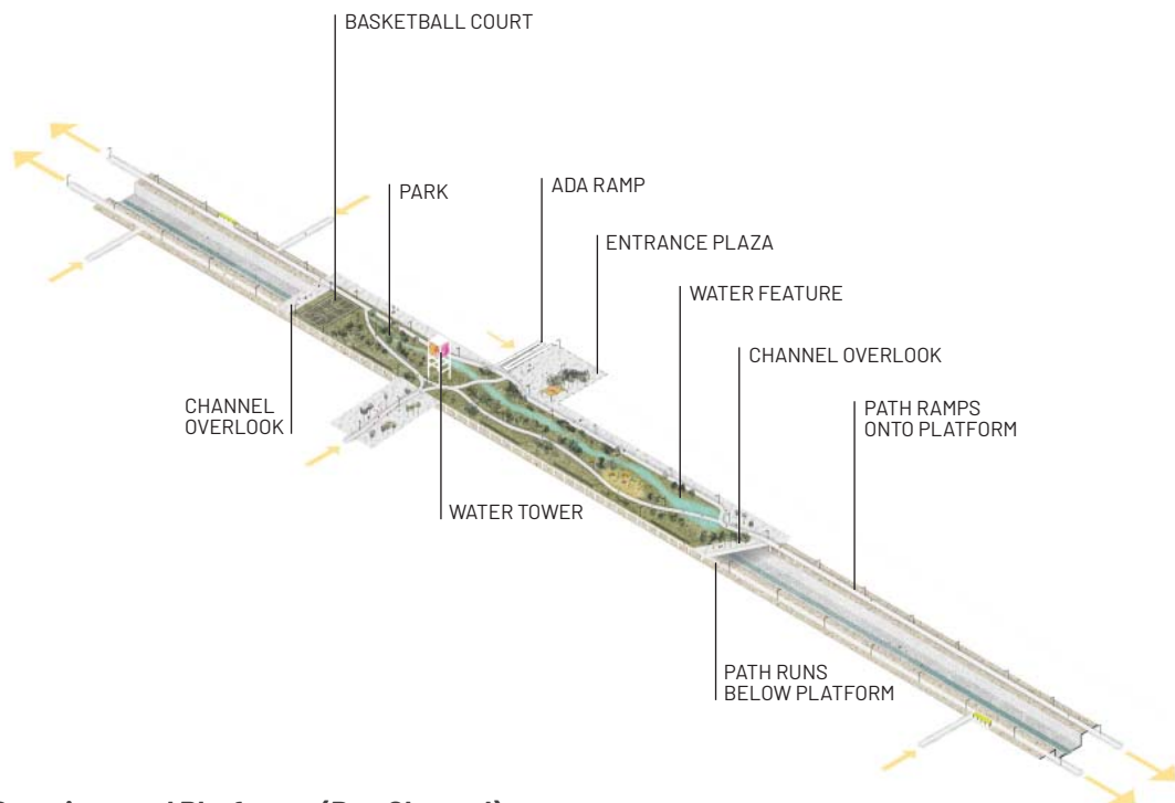
KOP 3 Crossings and Platforms (Box Channel)
