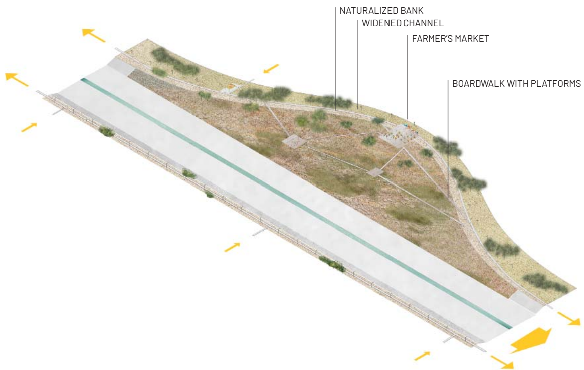
KOP 5 Floodplain Reclamation (Trapezoidal Channel)
