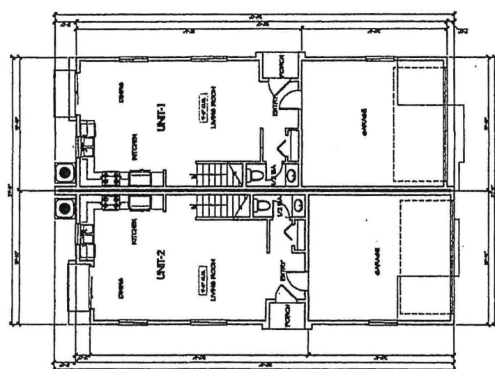
FLOOR PLAN SCALE 3/8"=1'-0"
