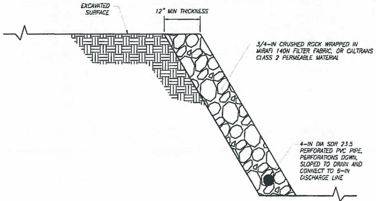
Figure 6 Bench Subdrain
