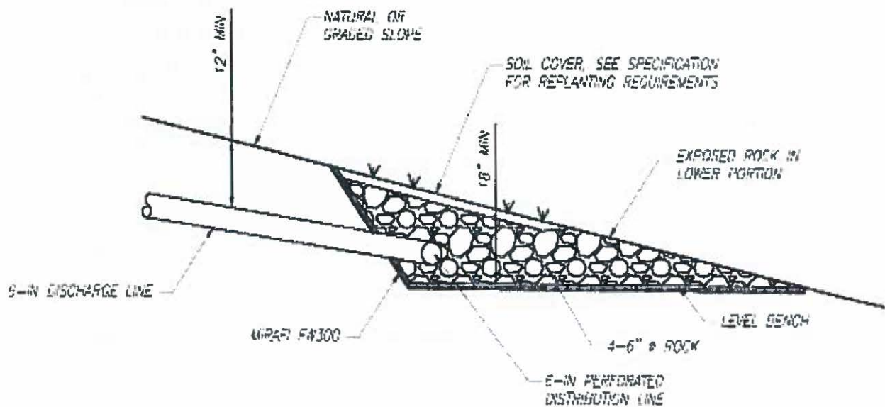
Figure 7 Riprap Energy Dissipator
