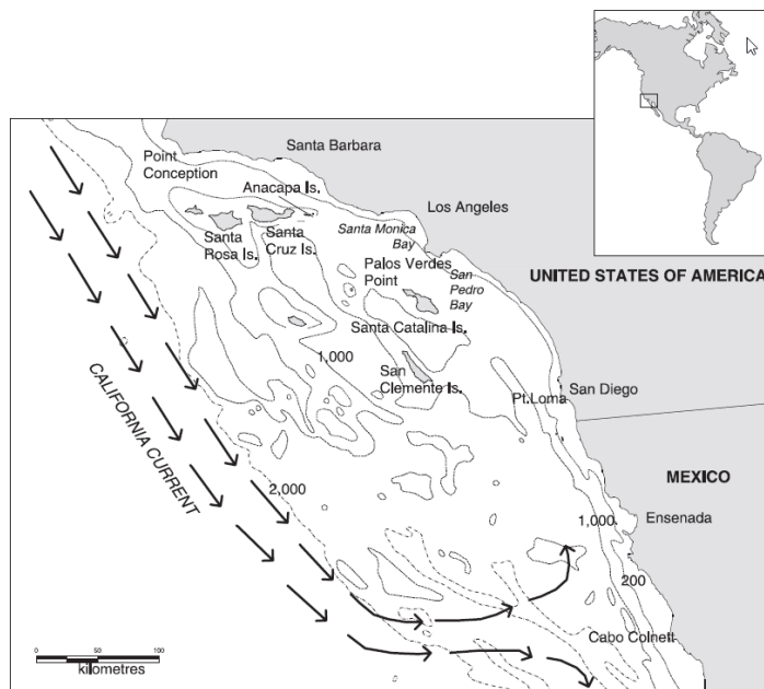
Figure 1. Map of the southern California, including general circulation patterns in the SCB (after Hickey 1993)
