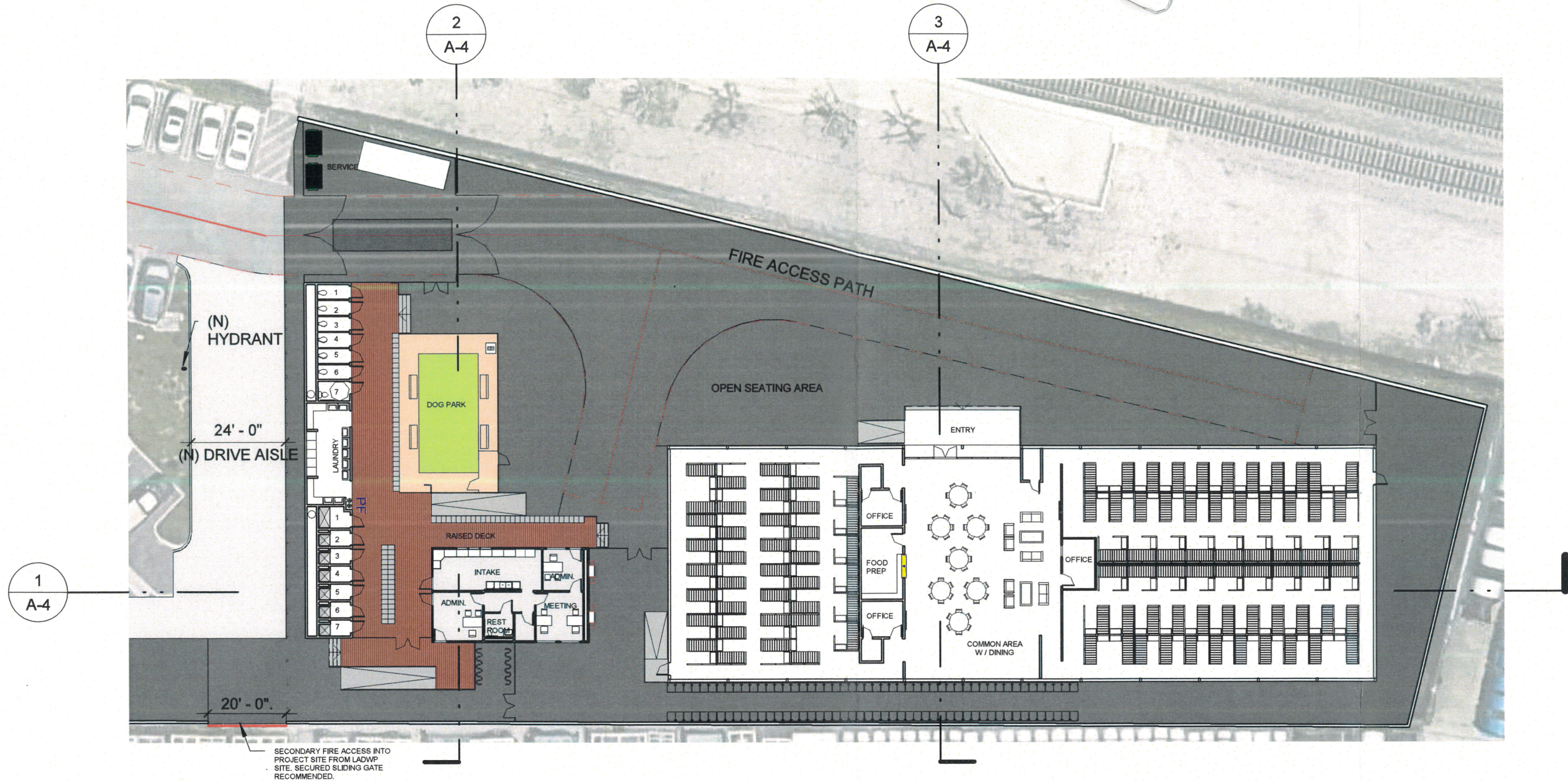
2 FIRST FLOOR PLAN 1" = 30'-0"
