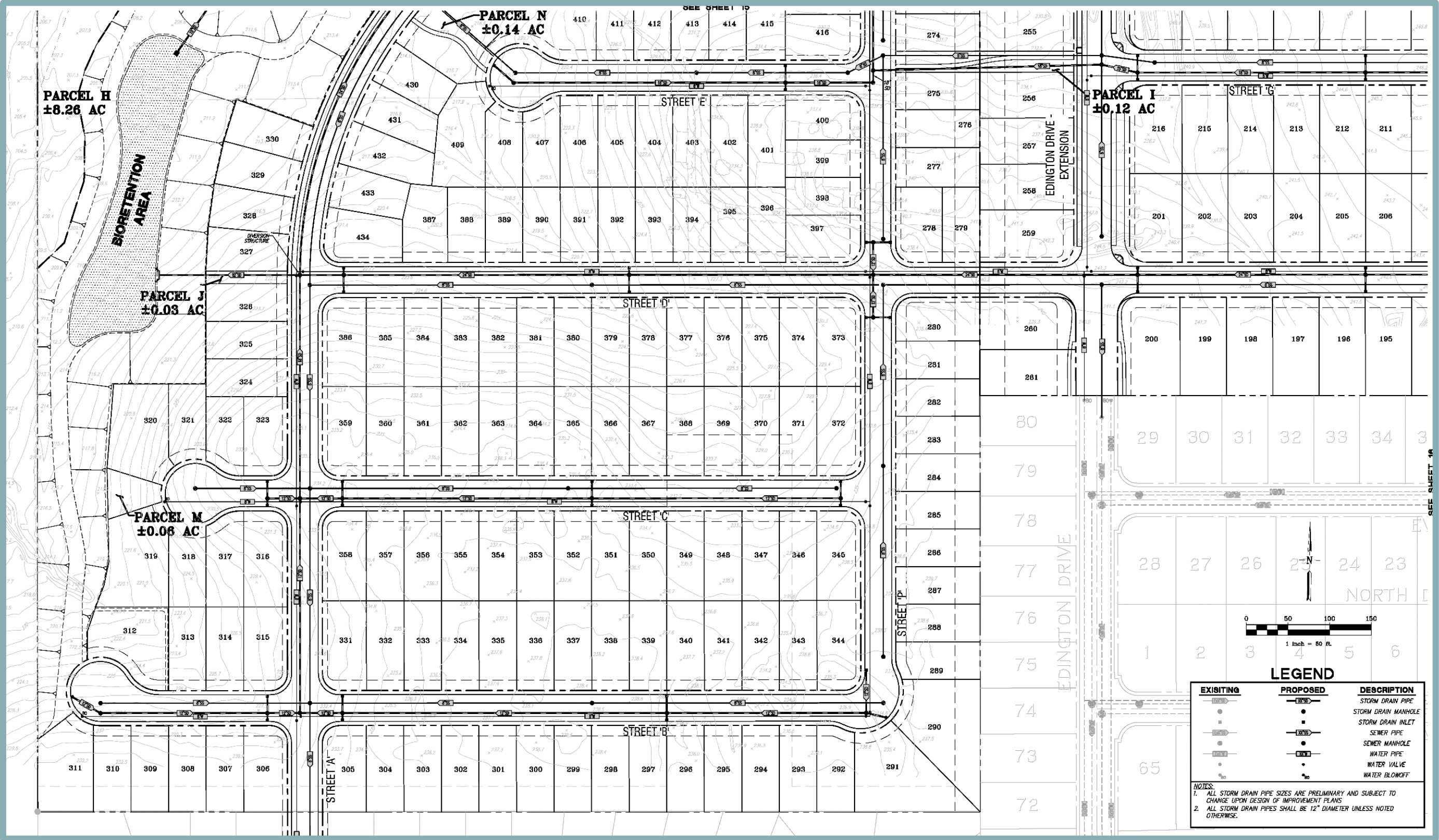
Figure 8 Preliminary Utilities Plan
