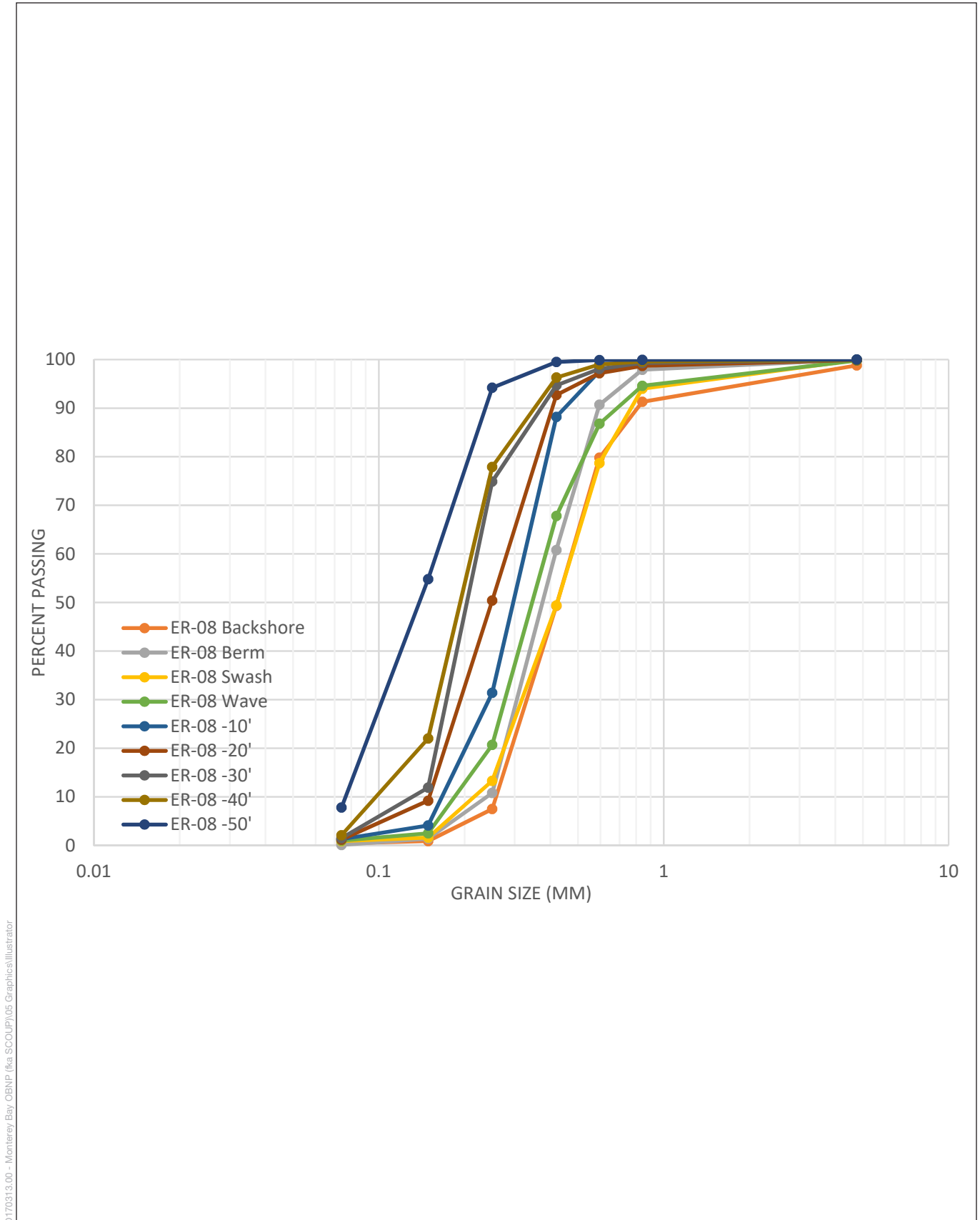
Figure 18 Example composite grain size envelope, for Marina Receiver Site
