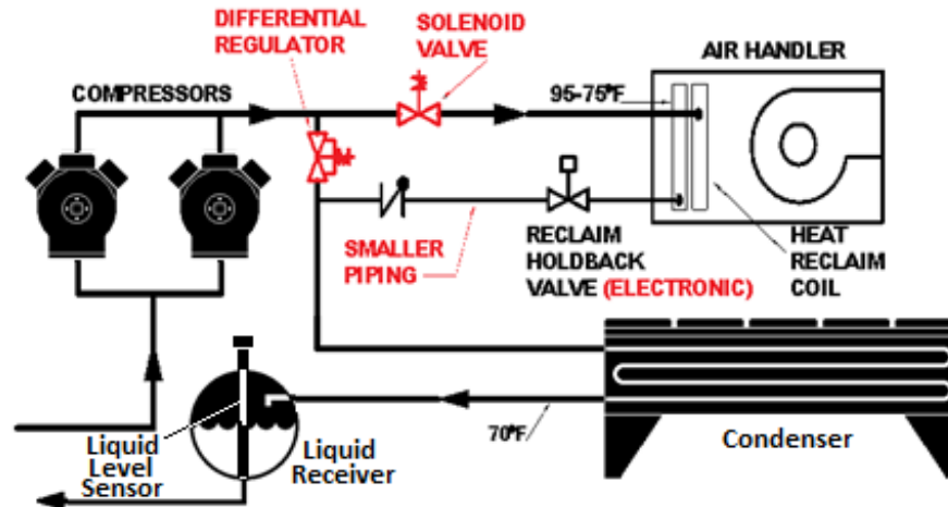
Figure 10-22: Direct-Condensing Configuration Showing Differential Regulator, Solenoid Valve, Electronic Holdback Valve
