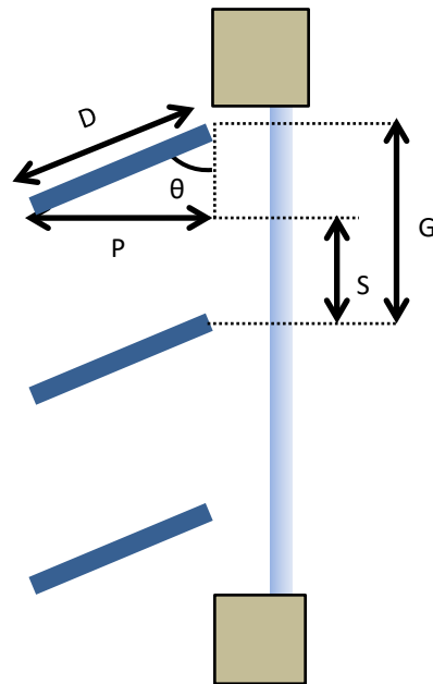
Figure 3-27 Projection Factor for Horizontal Slats
