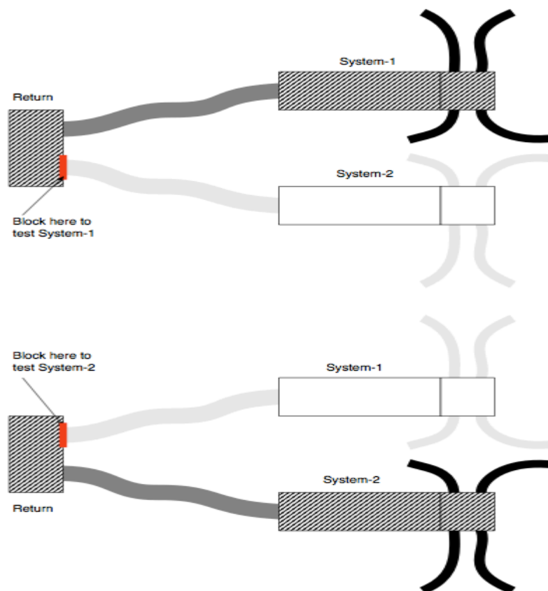
Figure 4-12: Example of Two Duct Systems with a Common Return
