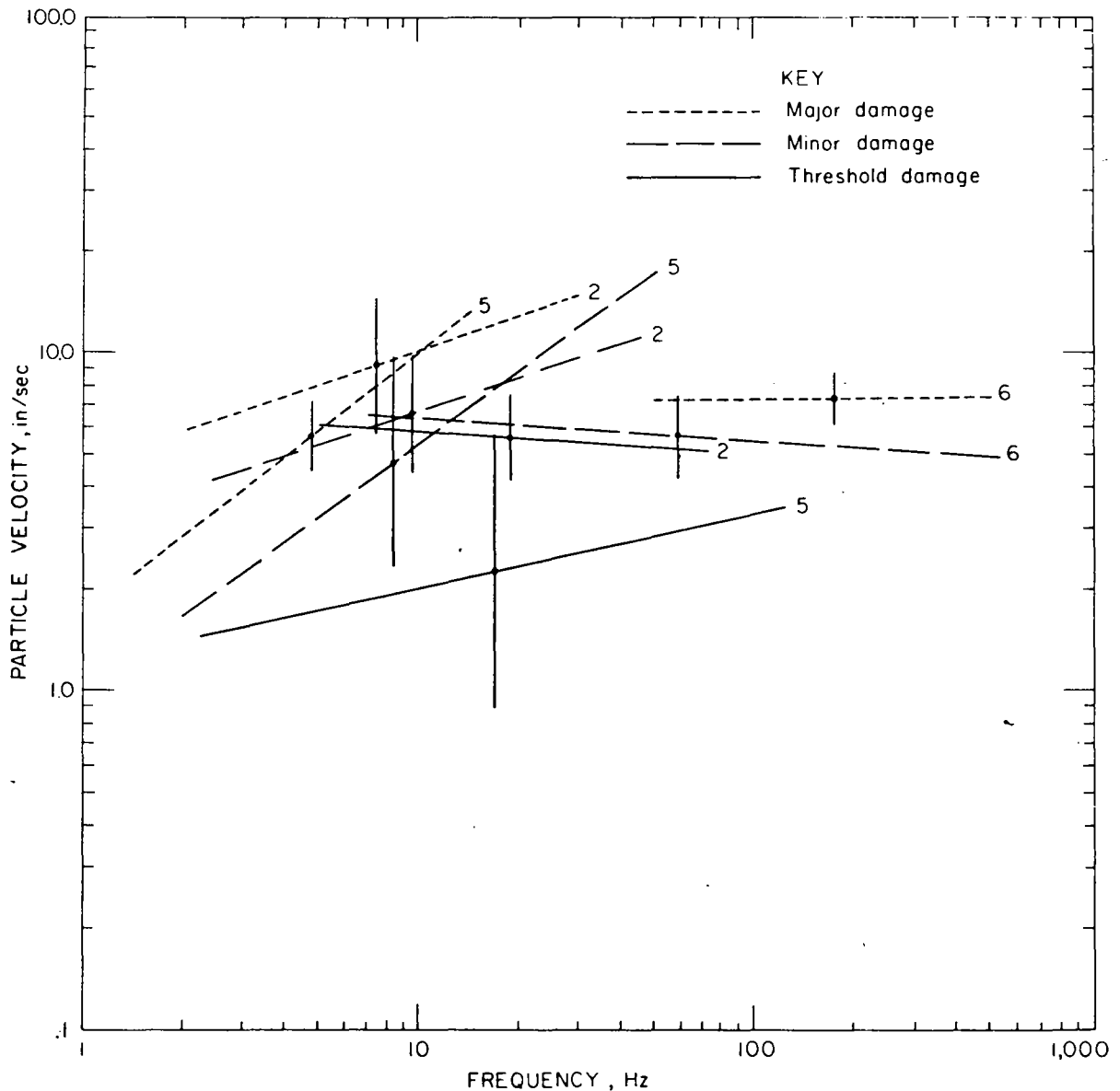
Figure 53.—Velocity versus frequency for the various damage data sets, mean and variance analysis. Sets are given in table 11.
