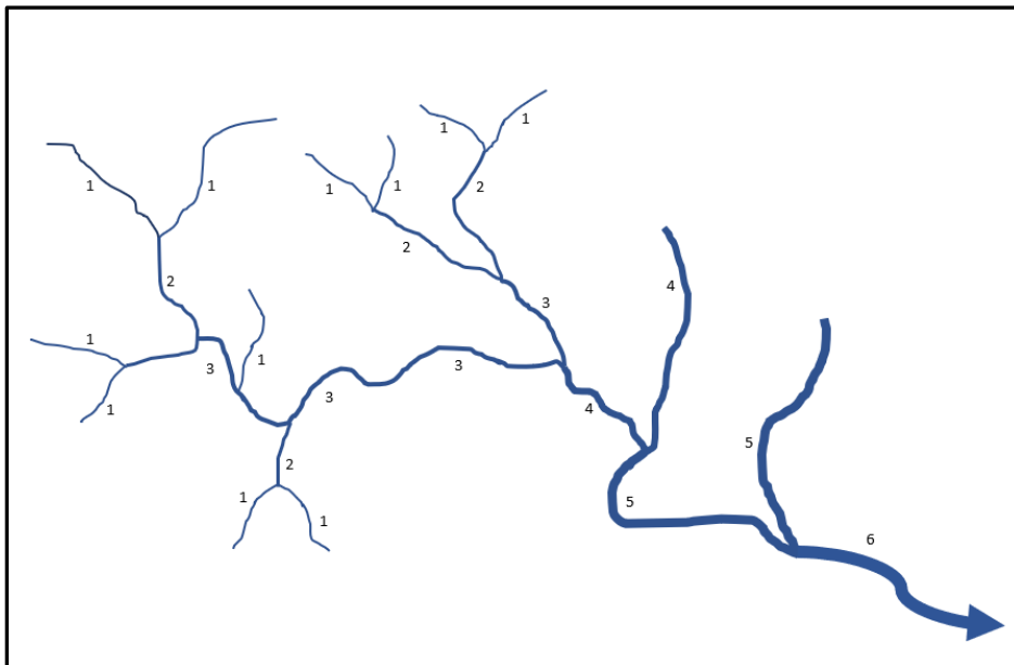
Figure A.C.5-3. Strahler Stream Order System
