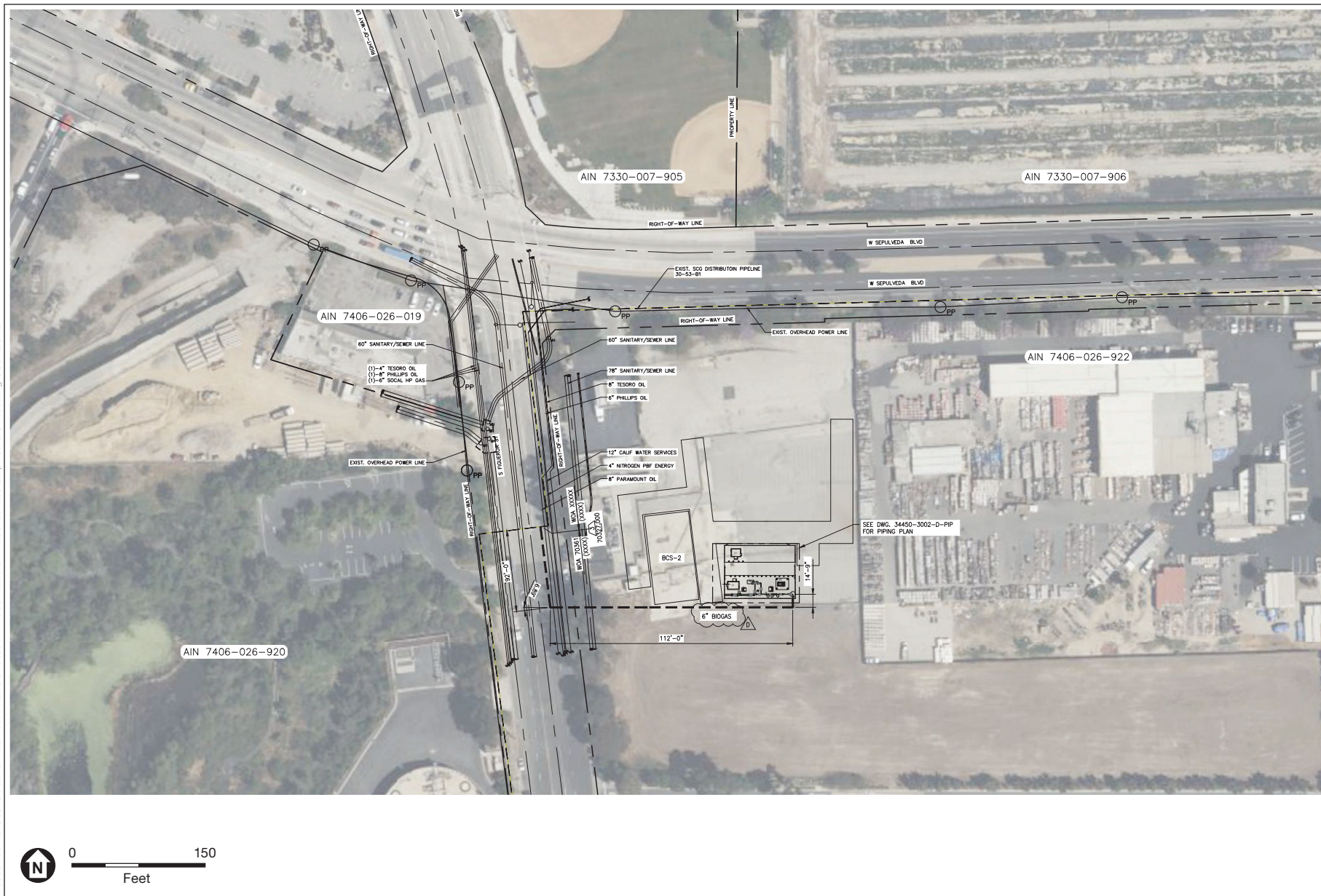
Figure 3 Proposed SoCalGas POR Facility and Pipeline Plan
