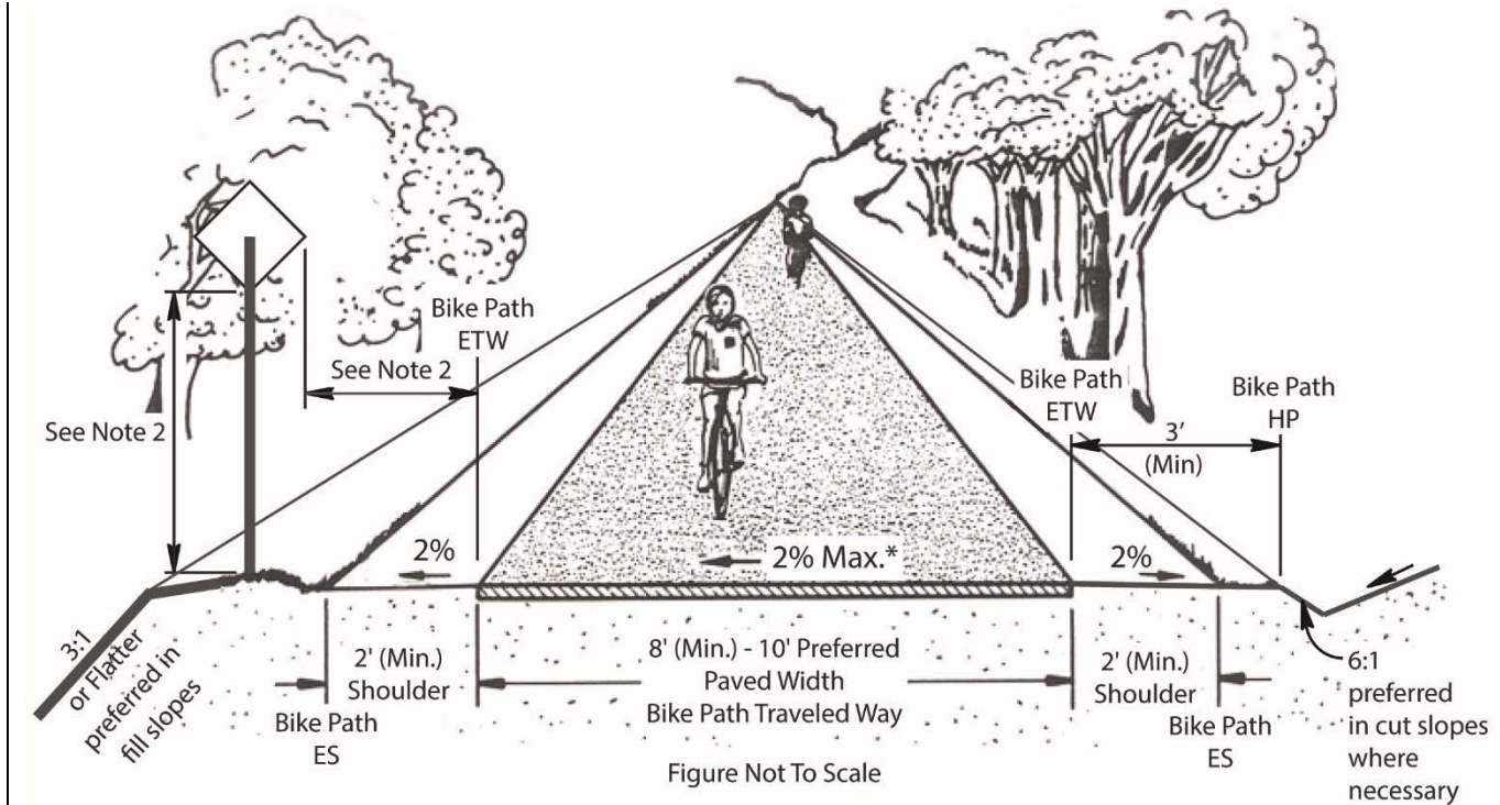
Figure 1003.1A Two-Way Class I Bikeway (Bike Path)
