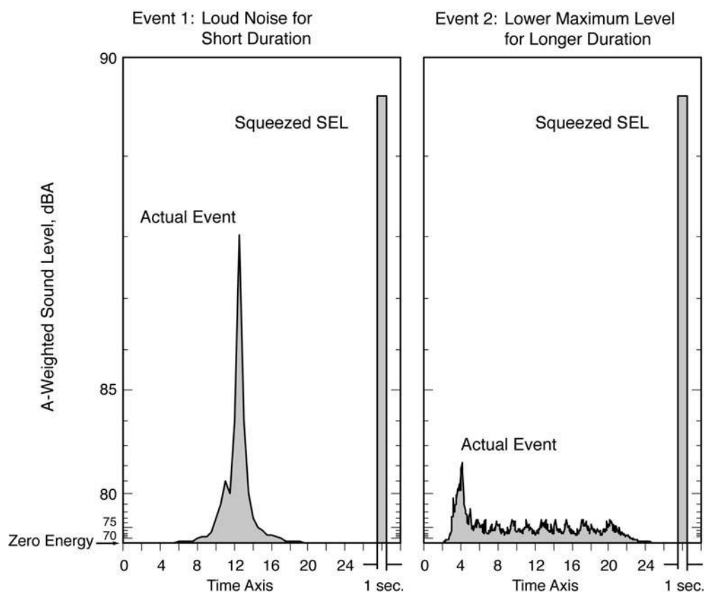
Figure B-8 An Energy View of Noise Events
