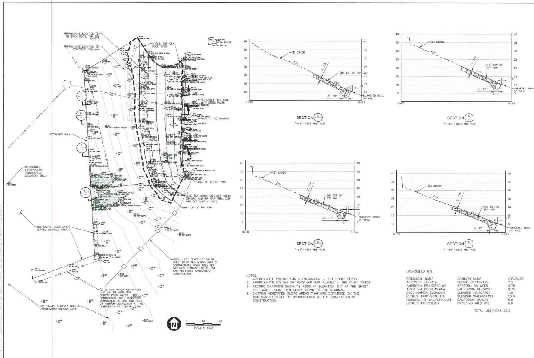
Figure 3 Site Plans and Cross Section
