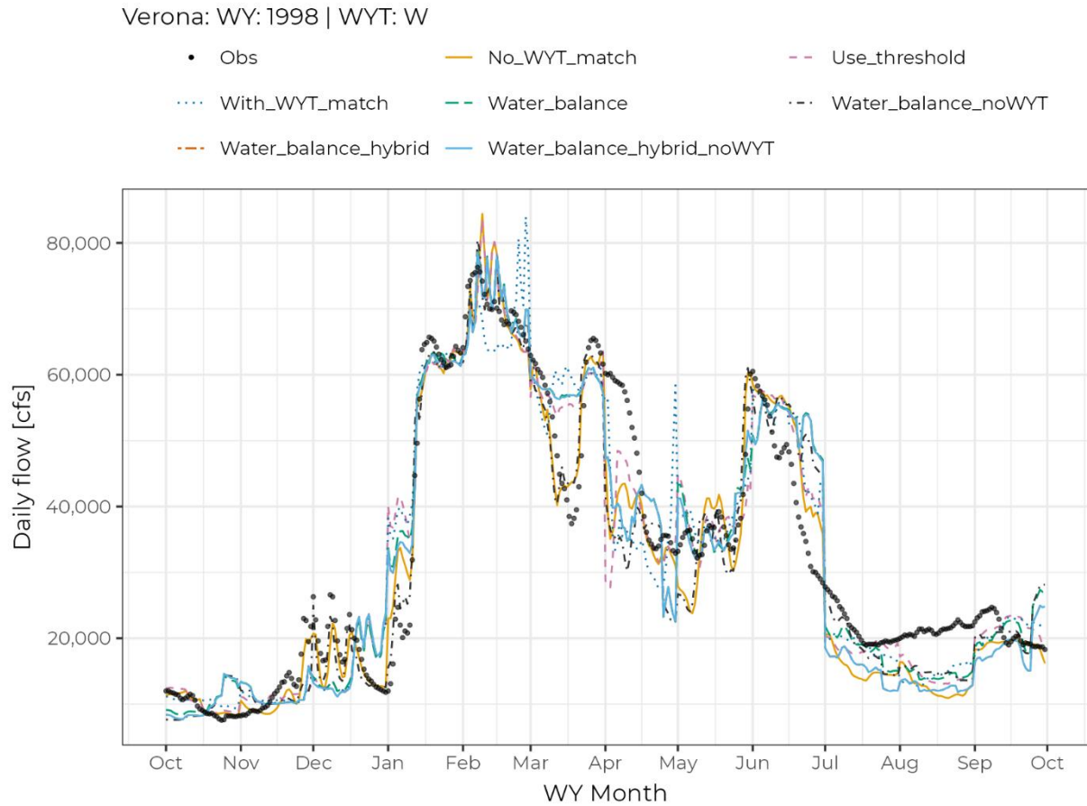
Figure 5A7-4. Daily simulated CalSim II flows using different daily pattern generation methods compared to observed flow (black dots) in the Sacramento River at Verona station in WY 1998.
