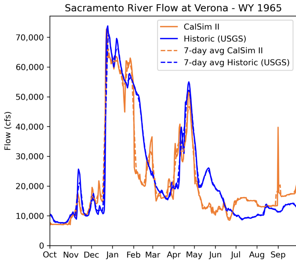
Figure 5A7-17. Sacramento River Flow at Verona in WY 1965 - Historic vs CalSim II (No Action Alternative 0111221).
