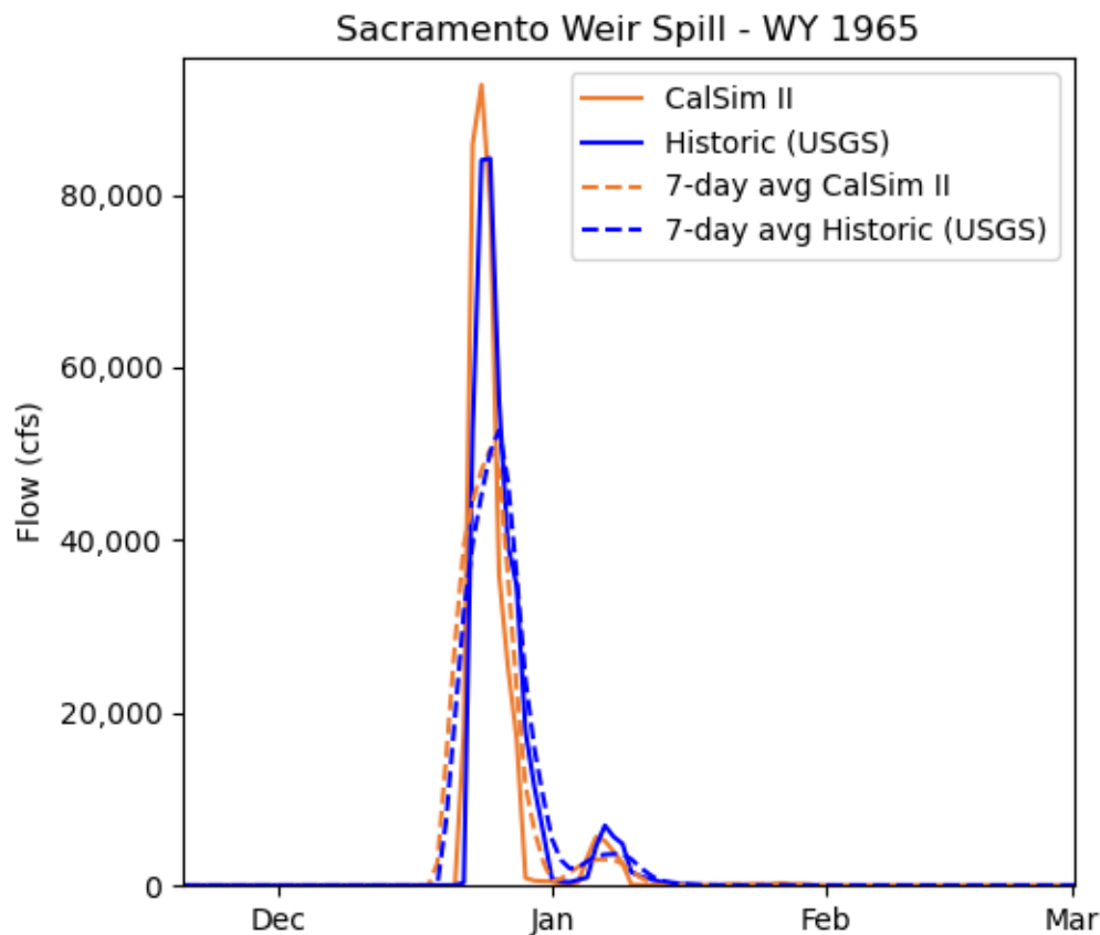
Figure 5A7-18. Sacramento Weir Spill in WY 1965 - Historic vs CalSim II (No Action Alternative 011221).
