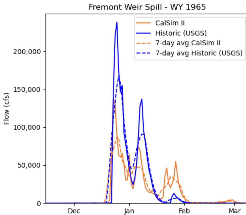
Figure 5A7-16. Fremont Weir Spill in WY 1965 - Historic vs CalSim II (No Action Alternative 011221).
